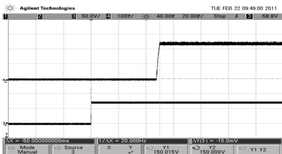
[Fig.11] Ch4: Vo, Ch3: Input voltage (20ms/div)
