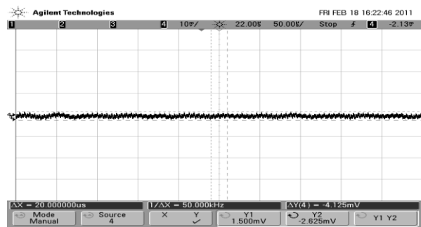
[Fig.6] Input reflect ripple current (0.5A/div)
