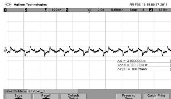
[Fig. 16] Output ripple & noise (100mV)
