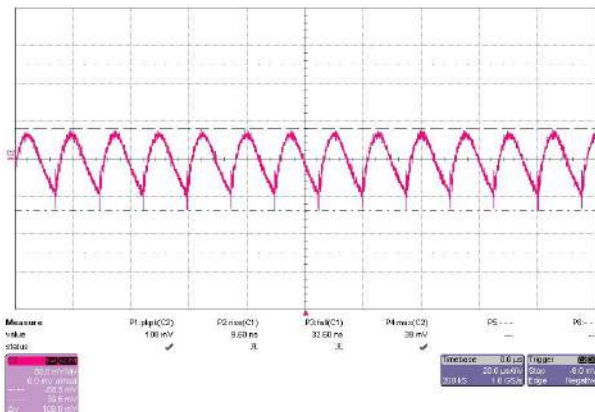
FS15-24 108.0mVpp
