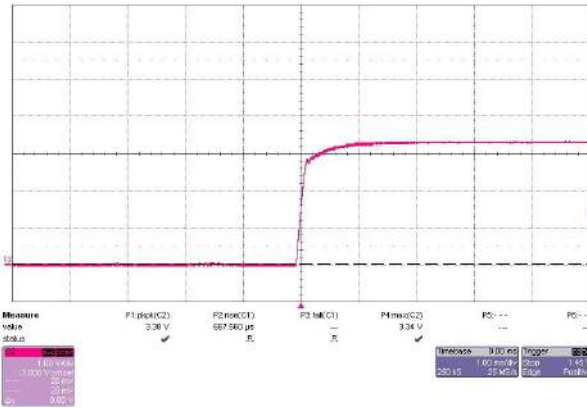
FS15-3R3 0V
