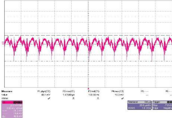
FS15-3R3 46.8mVpp
