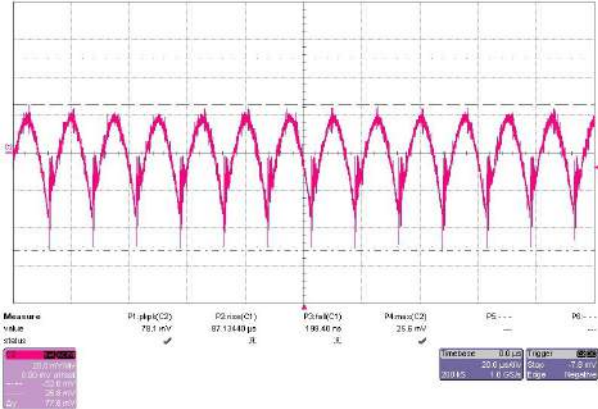
FS15-5 77.8mVpp
