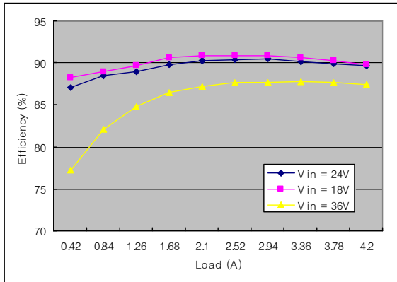
[Fig. 1] Efficiency for 18V, 24V and 36V input Voltage at 25°C, 400LFM.
