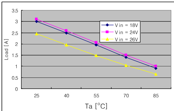
[Fig. 3] Thermal derating for 18V, 24V, and 36V
