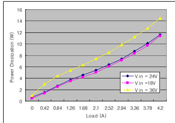
[Fig. 2] Power dissipation for 18V, 24V and 36V input voltage at 25°C, 400LFM.
