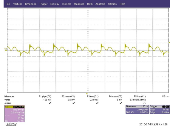
[Fig.4] Output voltage ripple & noise(100mV/div Bandwidth : 20MHz)
