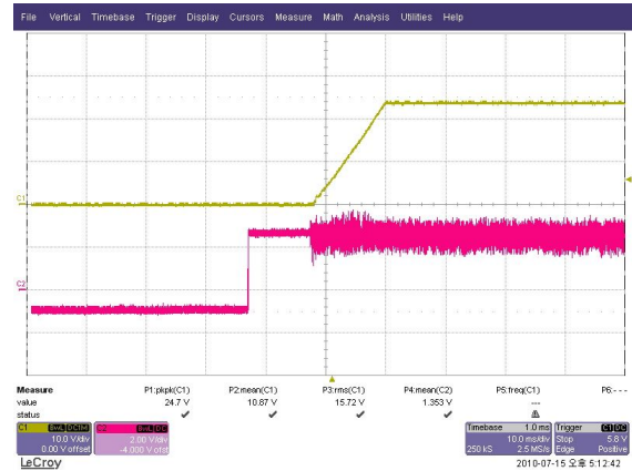
[Fig.6] Ch2: V_o , Ch3: On/off input(10ms/div)
